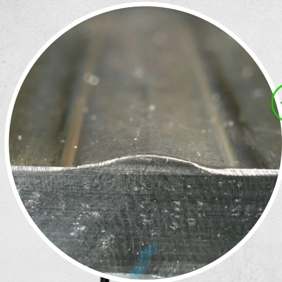
Stainless Steel Tank T: 10,0 mm Plasma Keyhole
